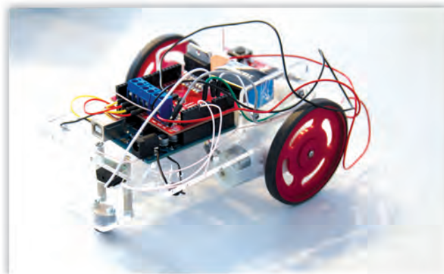
Robot commanded through virtual reality on computer, drawn up by the students and awarded the first prize, nationally and the third prize, internationally at INFOMATRIX contest, 2014.
